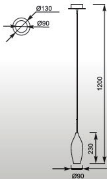
CHAMPAGNE Pendant 1. MD2101-1BL (black) 2. MD2101-1W (white) 1*E14 40W shiny black or white glass / metal chrome
